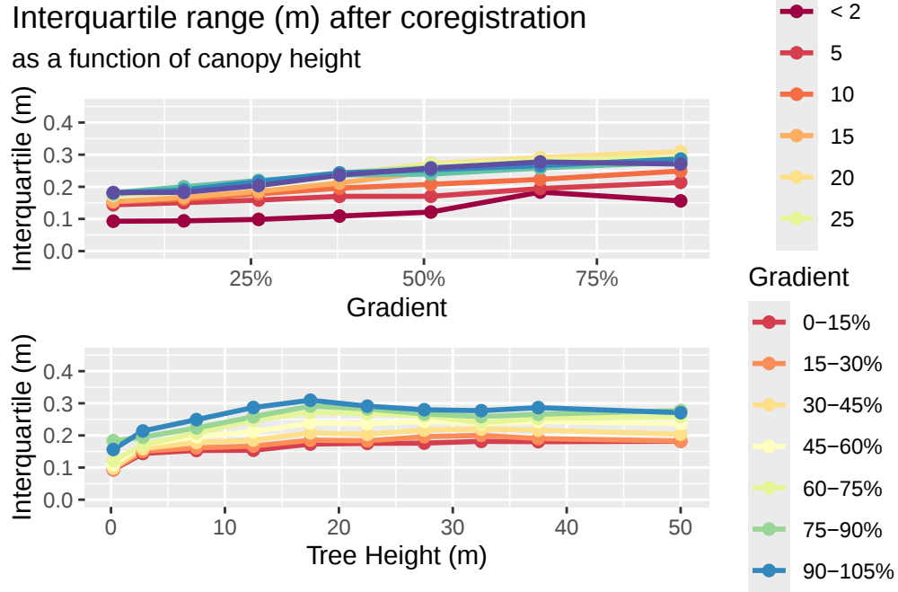
Figure 18: Variation of the interquartile range with changes in canopy height and hillslope gradient.
