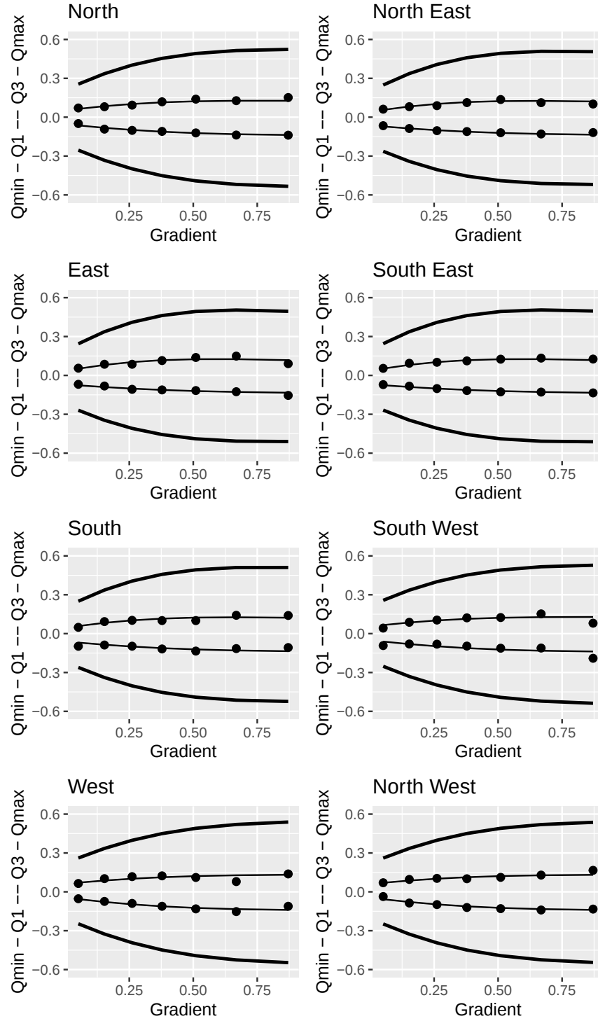
Figure 13: First and third quartiles (dots), polynomial fits (thin lines), and limits using Tukey's fences (k=1.5) after shifting the 2017 DTM.
