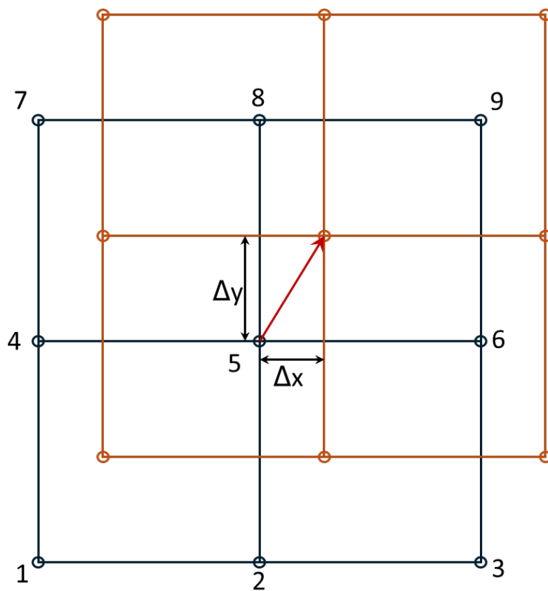
Figure 1: Shifting of the red DTM so that elevations at the black reference DTM center point (point 5) match as closely as possible.
