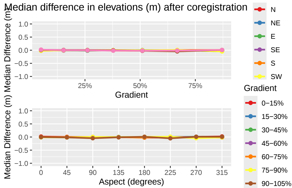
Figure 7: Median difference (m) in 2006 and 2017 DTM elevations after coregistration.
