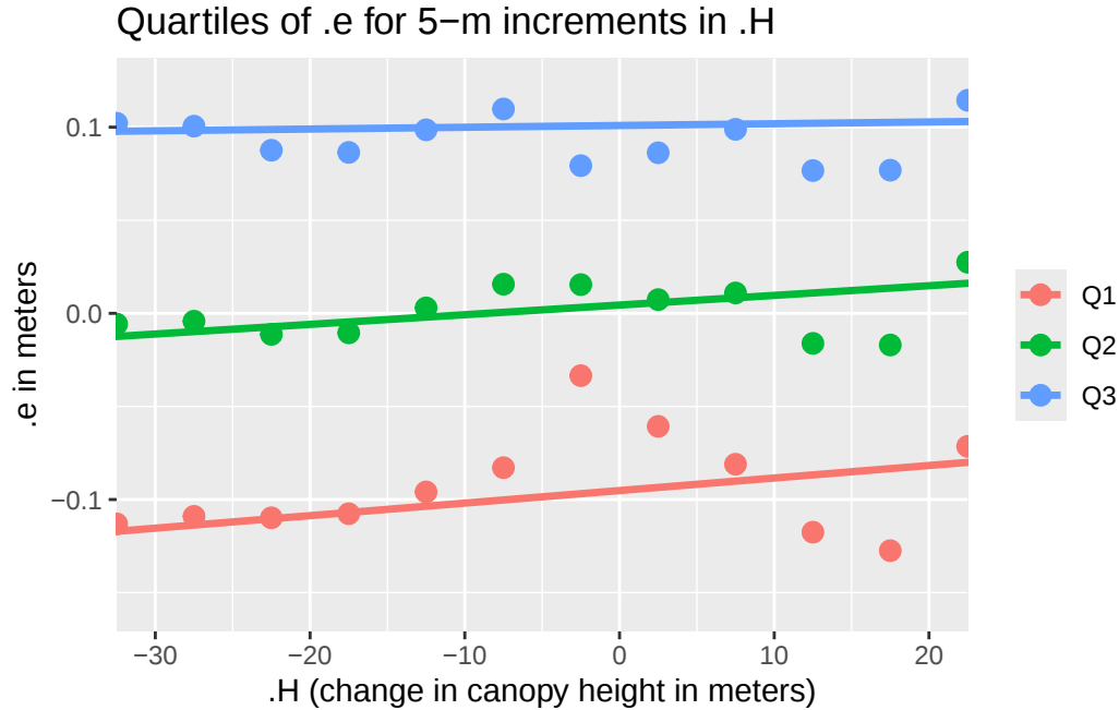
Figure 21: First, second, and third quartiles of \Delta e for increments of change in canopy height ( \Delta H ) between 2006 and 2007.
