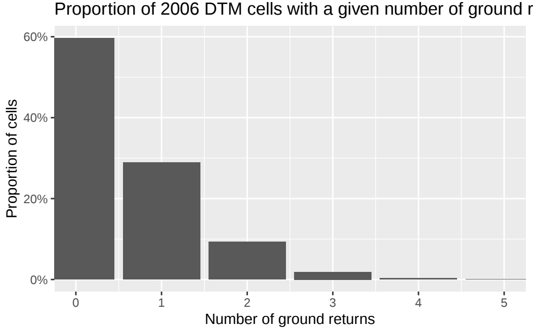
Figure 17: Proportion of 2006 DTM cells with a given number of ground returns
