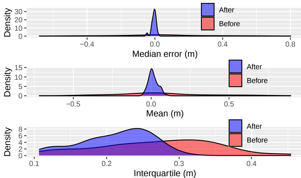
Density plots before and after coregistration
