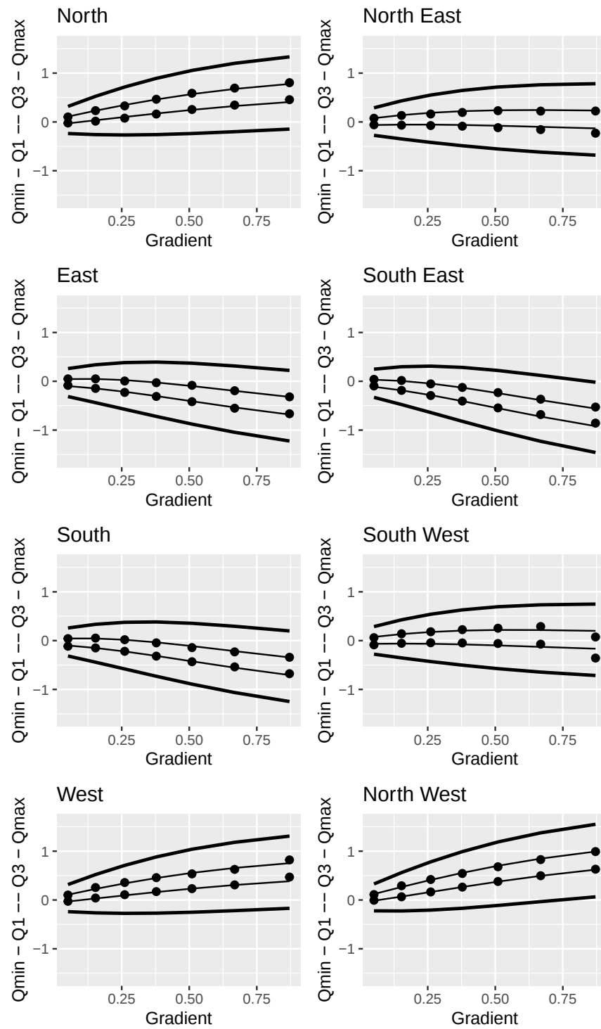
Figure 6: Hillslope gradient- and aspect-dependent level of detection (LoD). The dots indicate calculated first and third quartiles for each slope and aspect interval, the thin lines show the polynomial fit to those points, and the thick lines show the Tukey's fences using a k value of 1.5.
