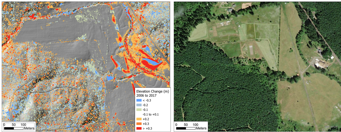
Figure 14: The left panel shows differences in DTM elevations after coregistration. The right panel shows an aerial photo view of the same area.
