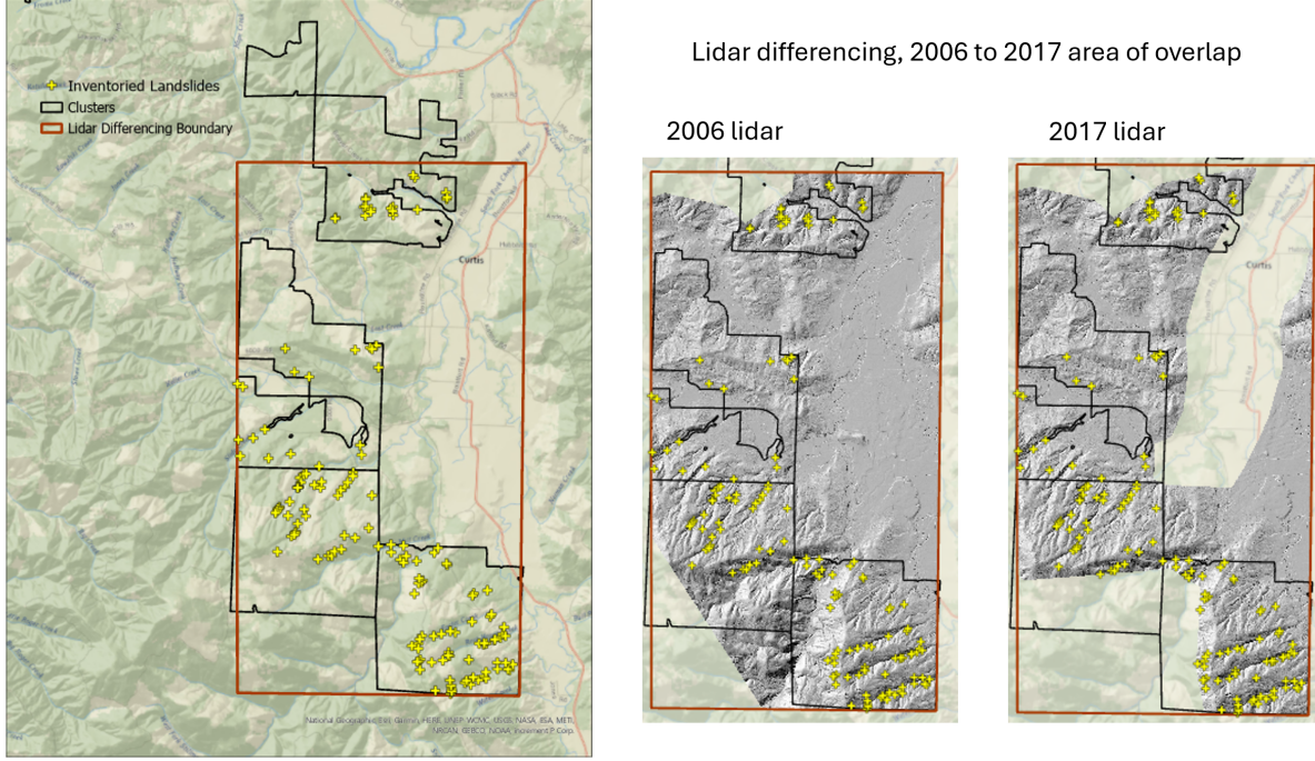
Figure 2: Site location and area of analysis.
