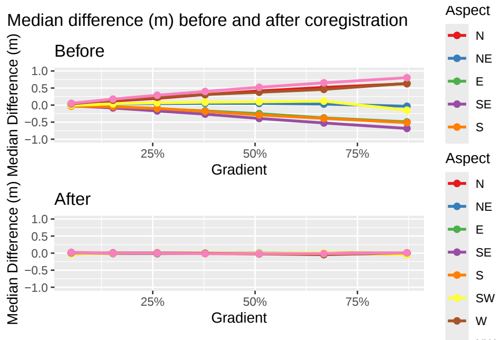
Figure 9: Median elevation differences (m) before and after coregistration.
