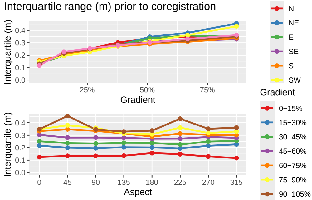
Figure 5: Interquartile range (m) of 2006 and 2017 DTM elevation differences prior to coregistration, after removal of apparent outliers.
