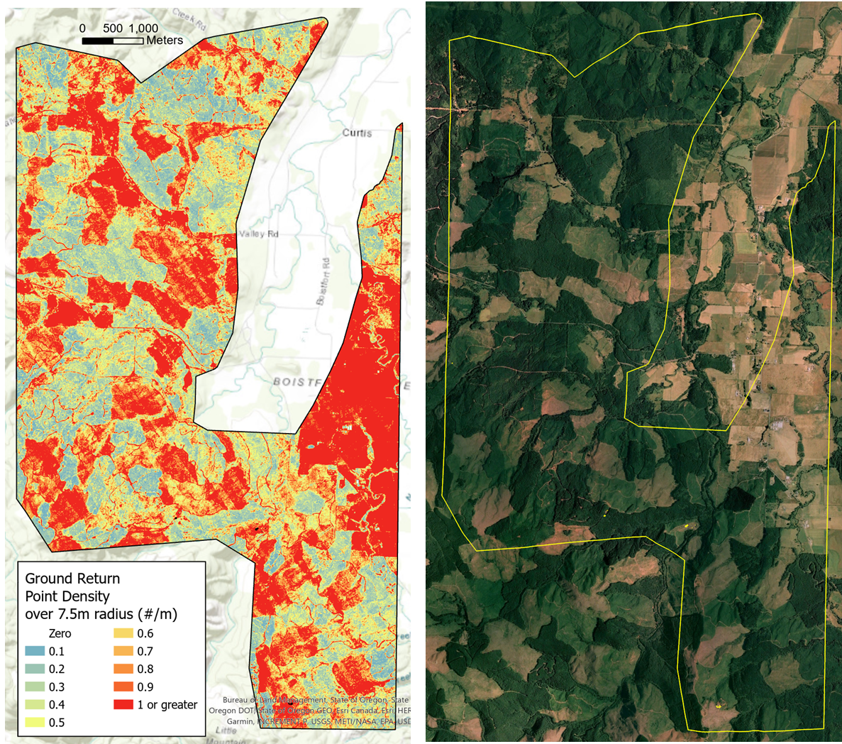
Figure 16: The left panel shows the ground-return point density for the 2006 lidar measured over a 7.5-m radius. The right panel shows an areal view of the area in the summer of 2006. Low point densities (blues) align with forested areas, high point densities (red) align with fields and clearcuts.
