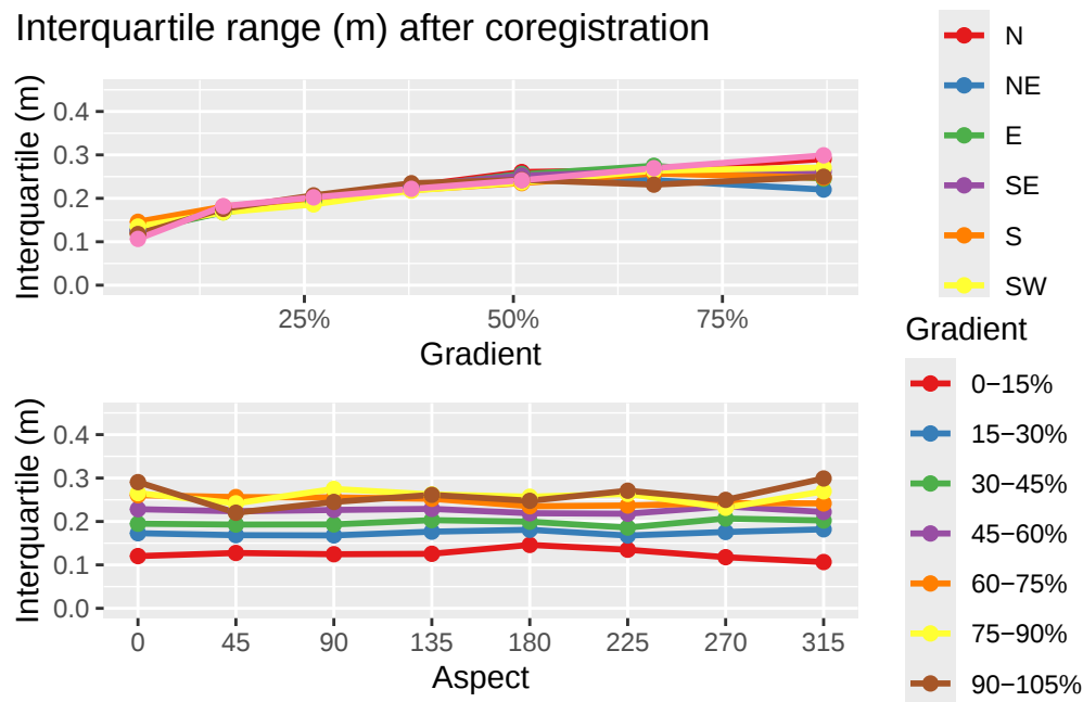
Figure 8: Interquartile range (m) of 2006 and 2017 DTM elevation differences after coregistration.
