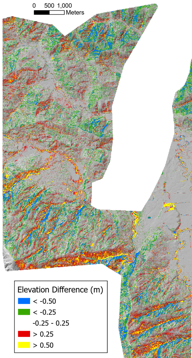
Figure 3: Elevation difference (m), 2006 to 2017 lidar overlap, draped on a shaded relief image
