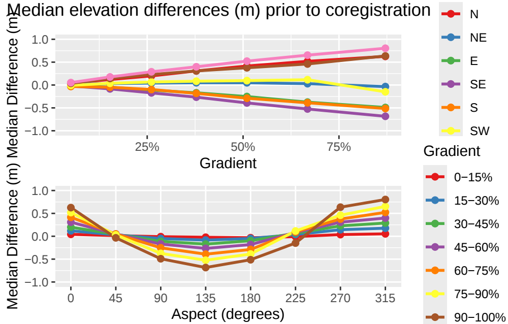
Figure 4: Median difference (m) in 2006 and 2017 DTM elevations prior to coregistration, after removal of apparent outliers.
