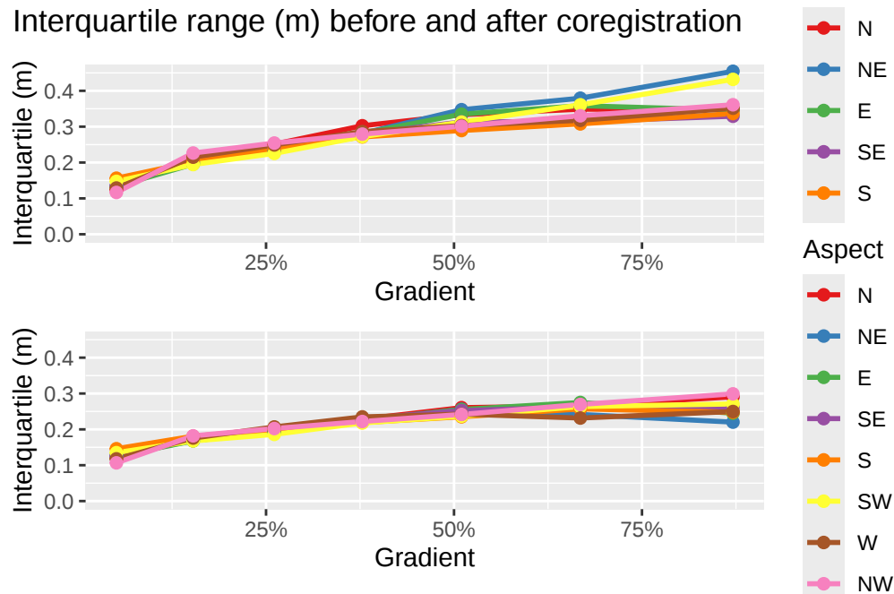
Figure 10: Interquartile range (m) before and after coregistration.
